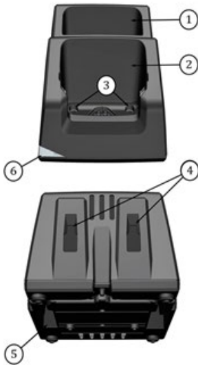
Figure 9 RCH-30 battery charger components
